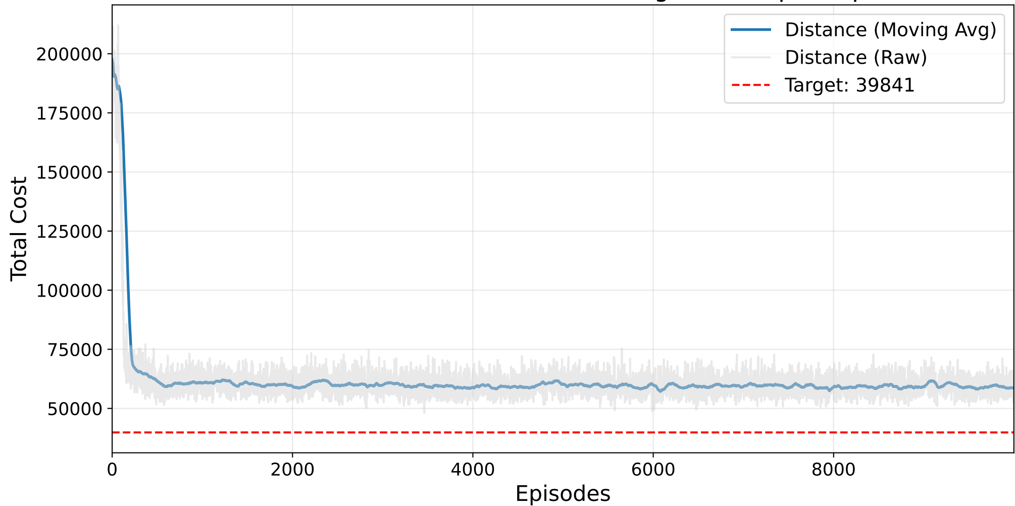
Final Masked AutoRL-SOP Training - kro124p.2.sop
